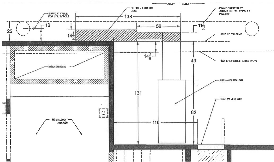
01 KITCHEN HOOD EXHAUST SCALE: 1/2" = 1'-0" (@ 11x17)
